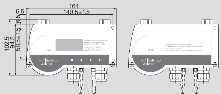
P29 with display
