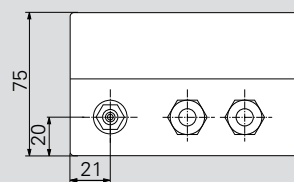
AD/BA 1000 with display
